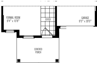
GROUND FLOOR | ELEV. A
