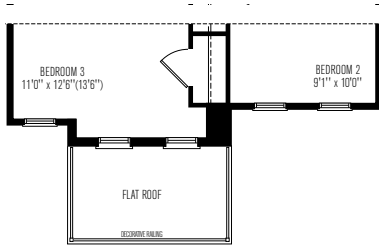
SECOND FLOOR | ELEV. A
