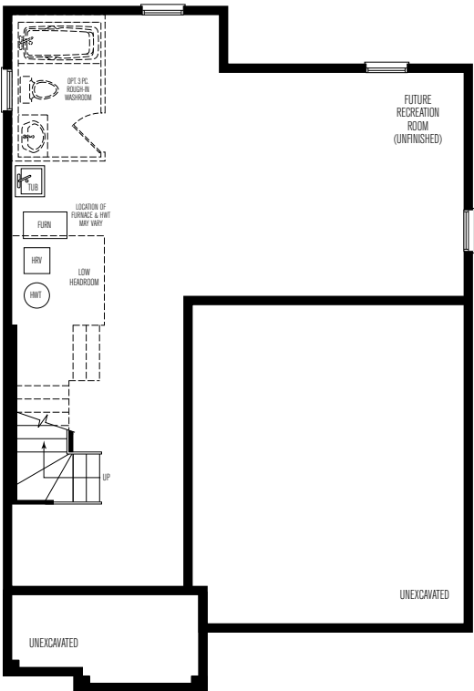
BASEMENT FLOOR | ELEV. A
