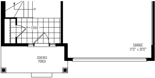
GROUND FLOOR | ELEV. B
