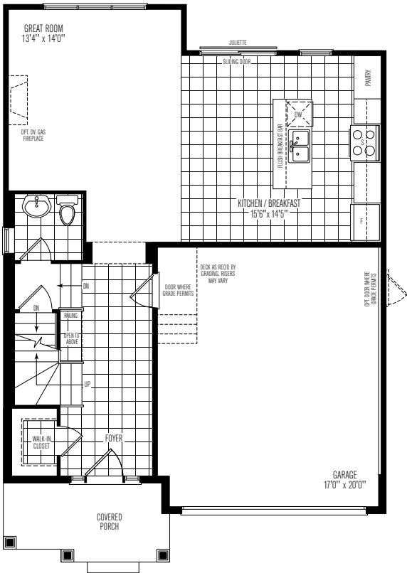
GROUND FLOOR | ELEV. A
