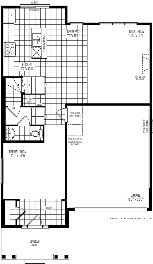
GROUND FLOOR | ELEV. A & B
