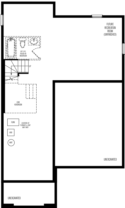
BASEMENT | ELEV. A & B
